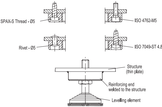
Assembling examples
